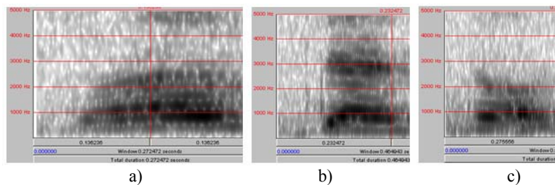
Figure 4. Spectrograms of the syllables /da/ (a) and /d j a/ (b and c). Anya, 2;1.
