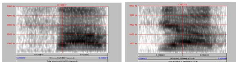
Figure 2. Spectrograms of the syllables /sa/ (on the left) and /s h a/ (on the right). Ksenya, 3;2.
