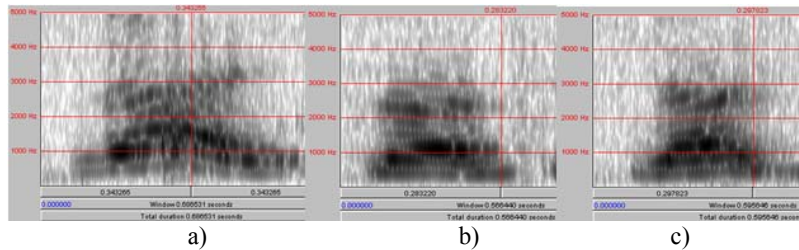
Figure 3. Spectrograms of the syllables /da/ (a) and /d j a/ (b and c). Ira, 1;3.
