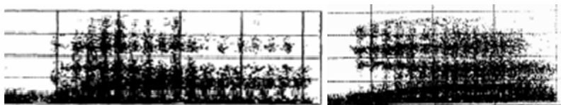
Figure 1. Spectrograms of the syllables / da / (on the left) and / b j a / (on the right) produced by an adult speaker of Russian (adapted from Kuznetsov 1997).
